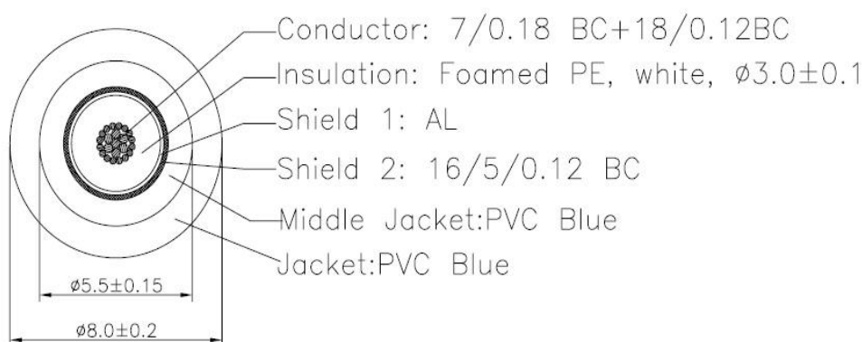
Cable construction
