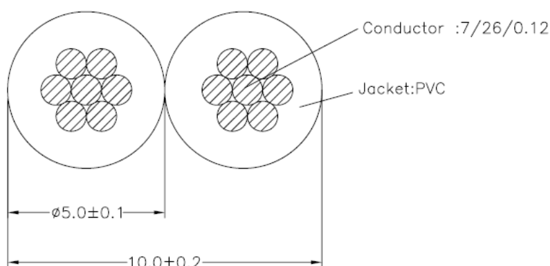
Cable Construction
